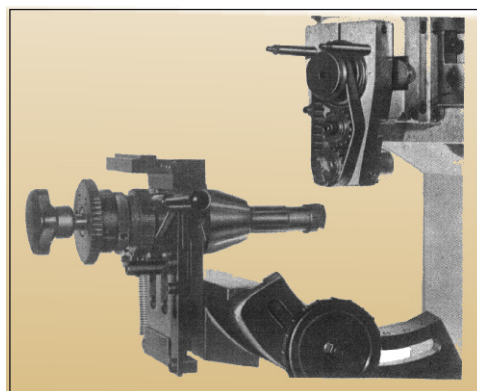
M-2 con divisor alianzas y portadiamantes 34 mm. Transmisión dentada (cod. SF020900). M-2 with rings divider and cutter head 34 mm. Toothed belt (cod. SF020900).
