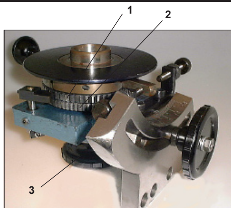
Cod. SF030700 P-15N Divisor horizontal P-15N Divider flat pieces
